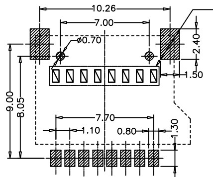
Recommended P.C.B Layout(Tolerance=±0.05) AS VIEW FORM COMPONENT SIDE
